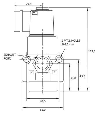
U10626 SERIES Dimensions shown are metric (mm)
