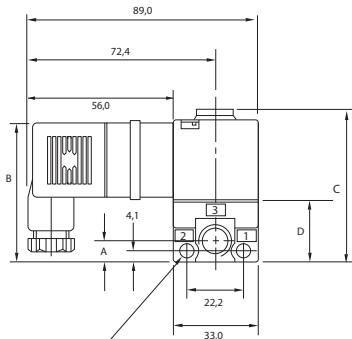
20311 SERIES Dimensions shown are metric (mm)
