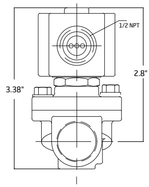
U10602/VAL SERIES Dimensions shown are inch (in)
